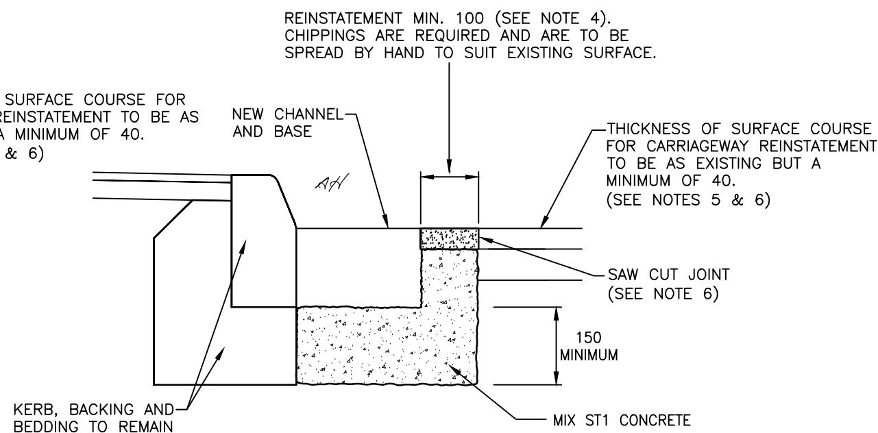
REPLACEMENT CHANNEL LAID ON NEW BASE
