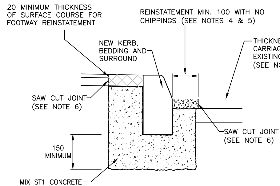
REPLACEMENT KERB LAID ON NEW BASE
