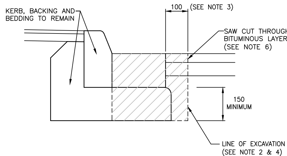
TAKE UP EXISTING CHANNEL AND BED
