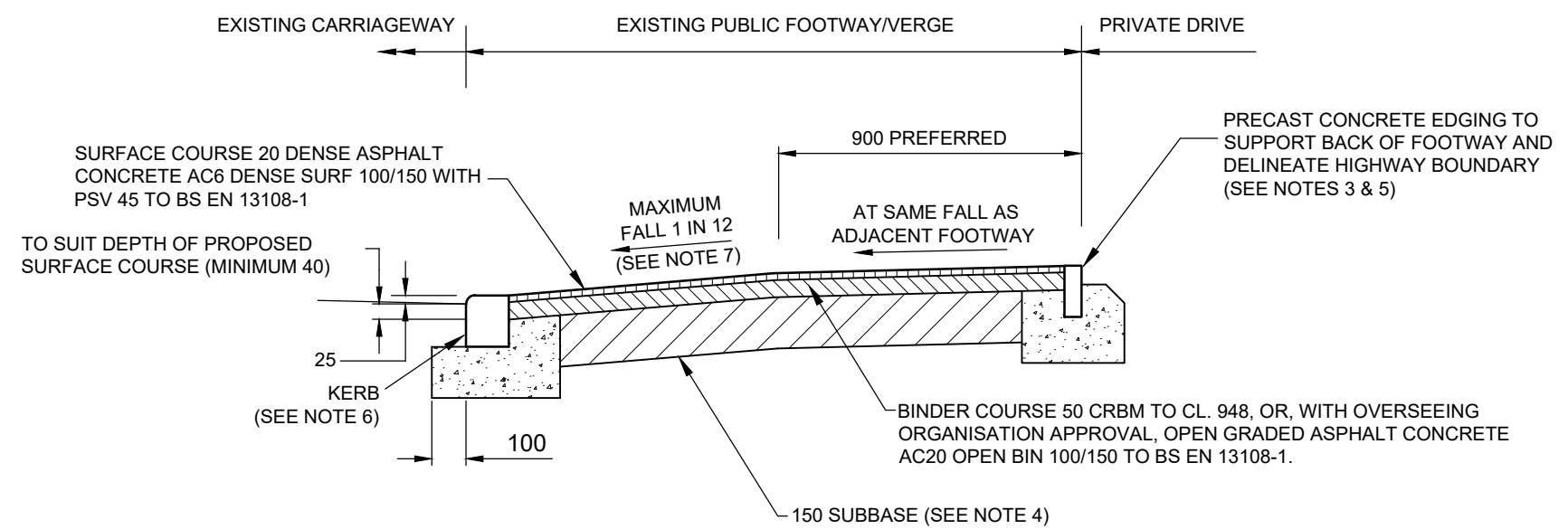
SECTION A-A FOOTWAY TYPE 1 - FLEXIBLE CONSTRUCTION
