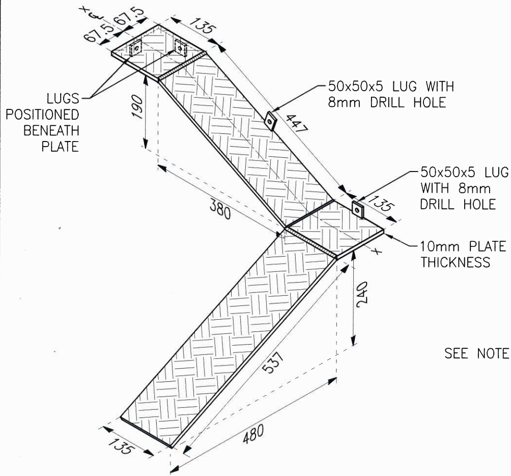
DETAIL E — ANIMAL ESCAPE RAMP SCALE 1:10
