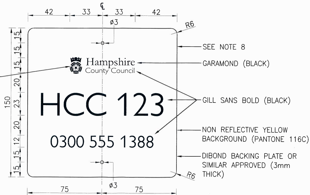
DETAIL F — CATTLE GRID PLATE SCALE 1:2
