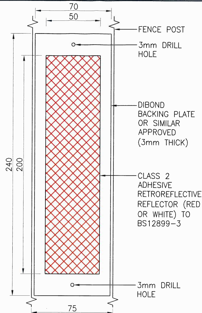
DETAIL D SCALE 1:2
