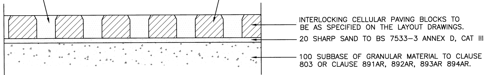
CELLULAR BLOCK FOUNDATION DETAIL TYPE 'B'
