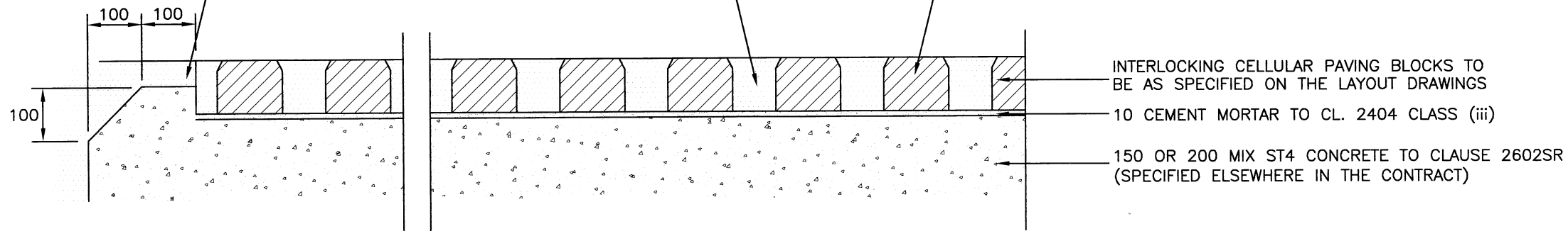
CELLULAR BLOCK FOUNDATION DETAIL TYPE 'A'
