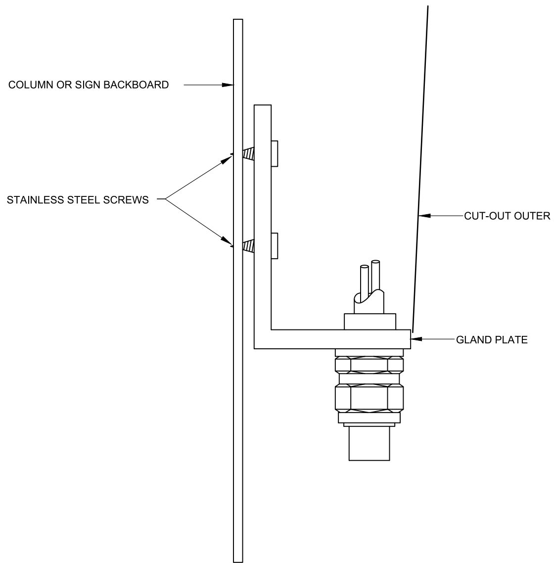
CABLE GLAND TYPES CW & CX
