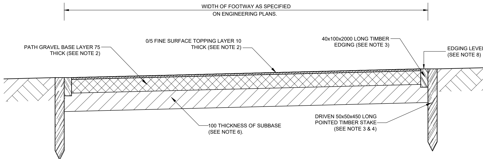
FOOTWAY TYPE 4 - RURAL
