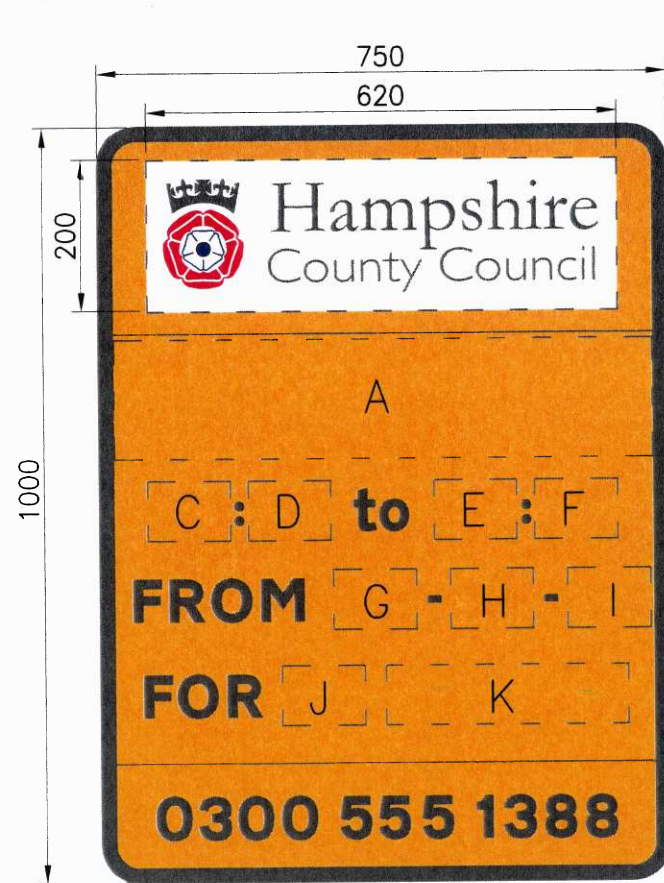
TYPE 2 SIGN FOR LAMP COLUMNS
