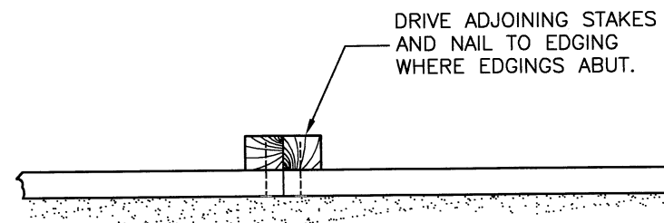
PLAN DETAIL 'A' (SEE NOTE 5)
