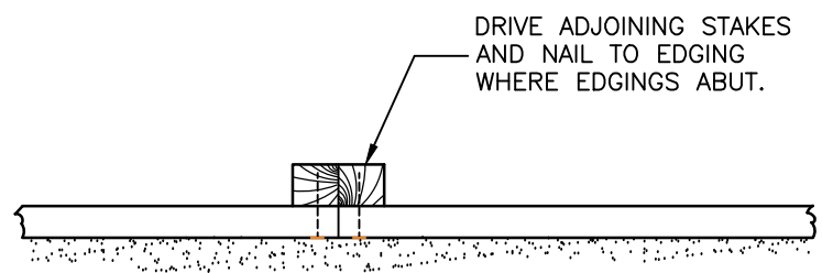
PLAN DETAIL 'A' (SEE NOTE 5)
