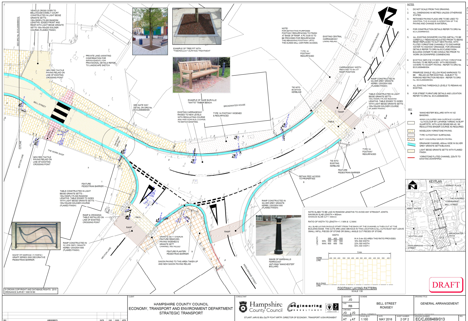
Layout Plan 1/2
