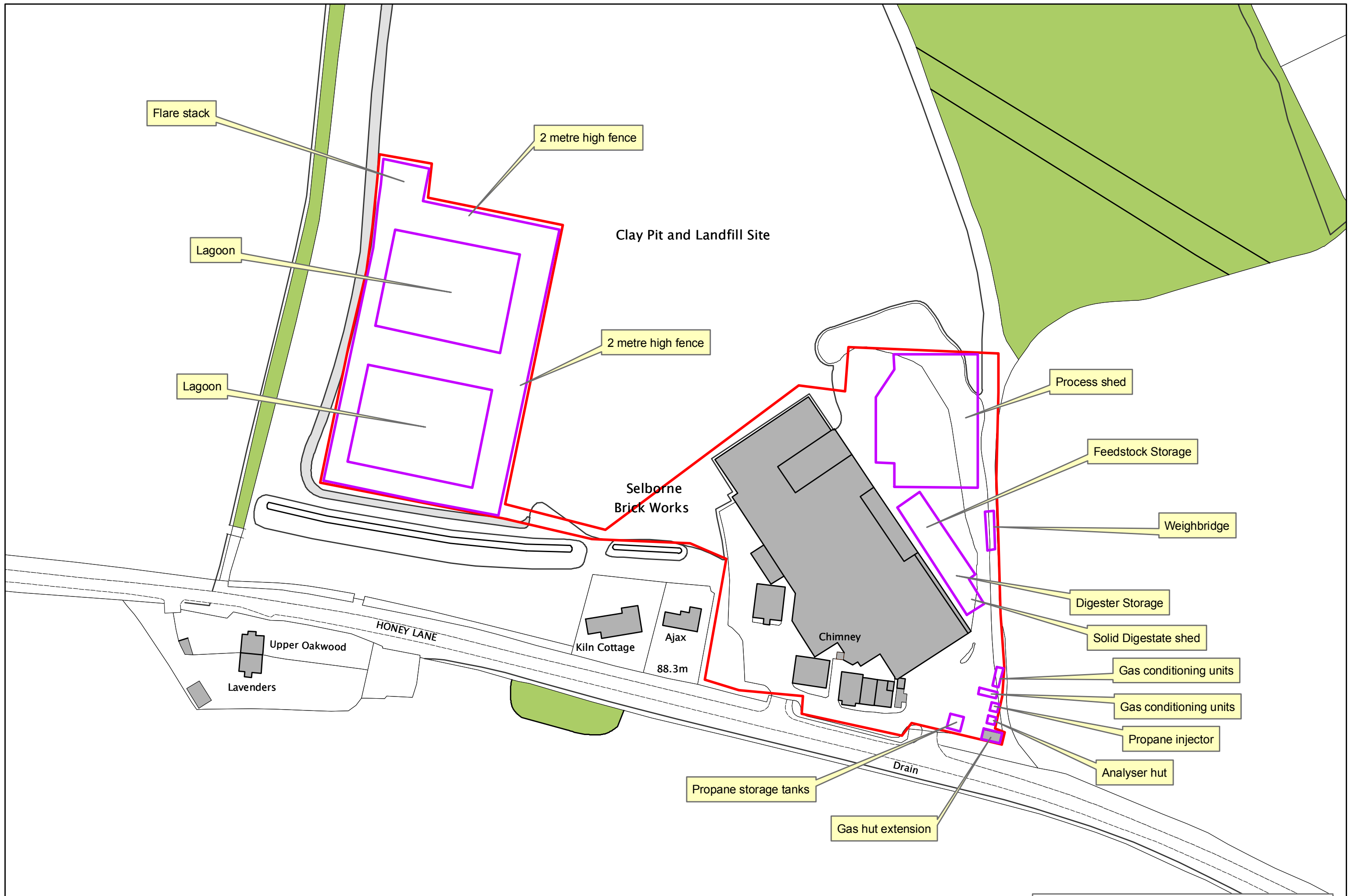
Selborne Brickworks AD Plant - Layout. Scale 1:1,250
