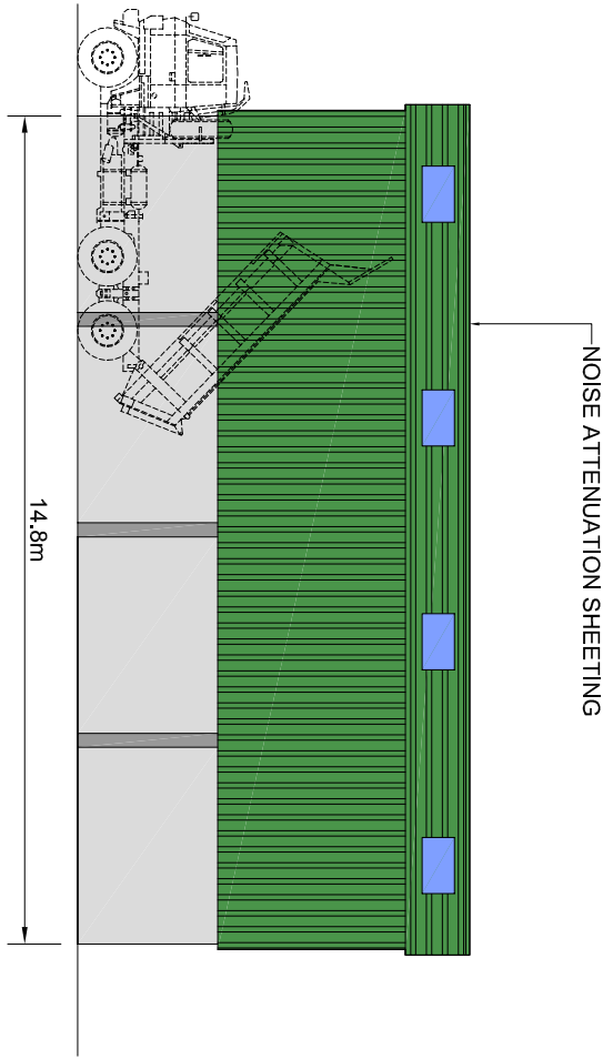
NORTH ELEVATION SCALE 1:150
