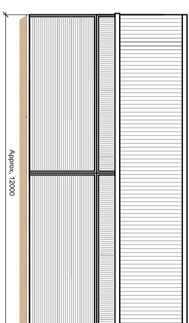
North Elevation
