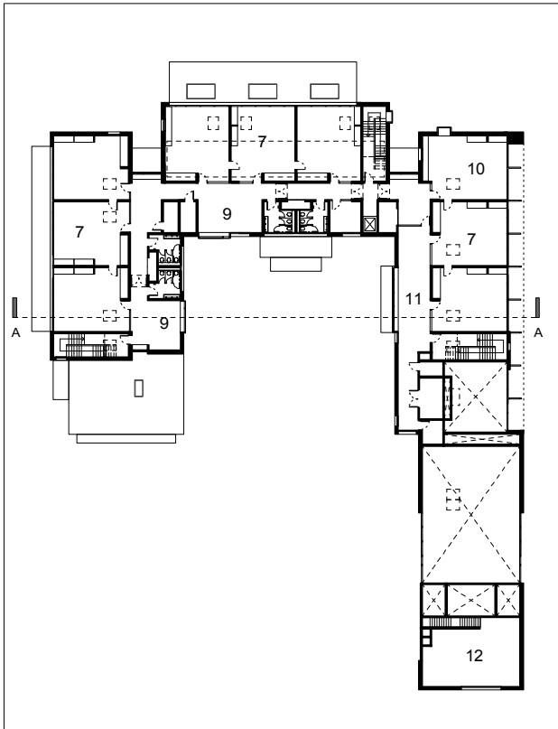
Proposed Primary School - First Floor Plan
