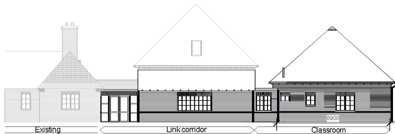
Existing Link corridor Classroom Proposed North Elevation @ 1:200
