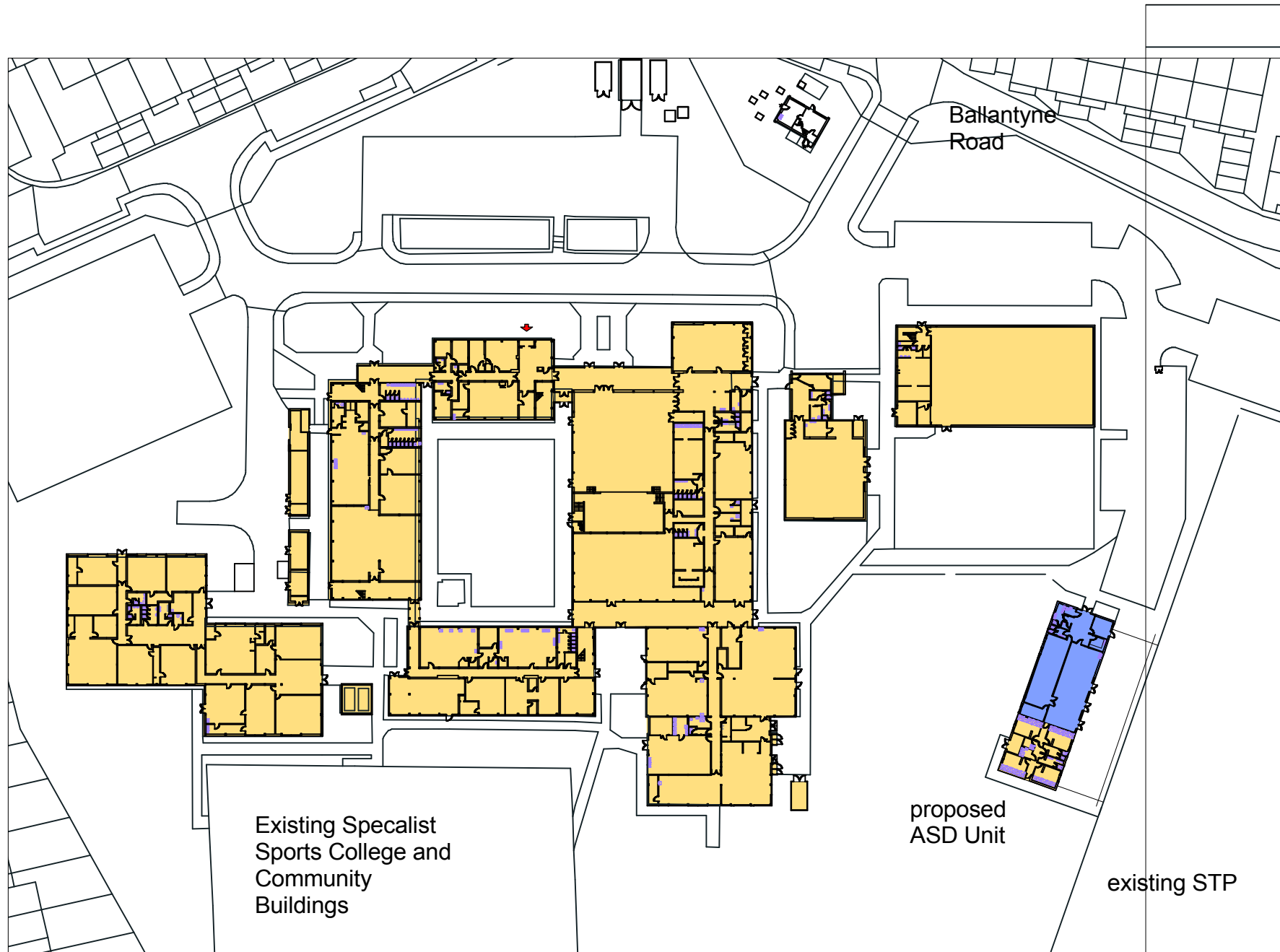
School Site Plan - Scale 1:1000
