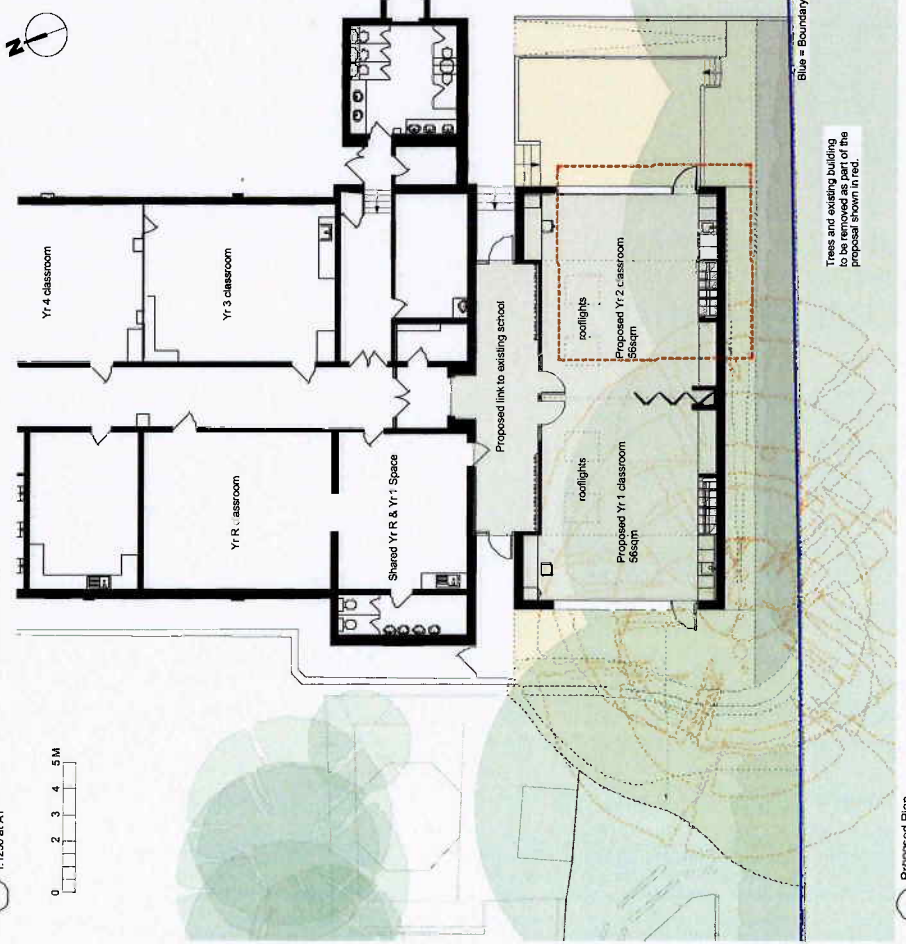
2 Proposed Plan 1:1100 at A1
