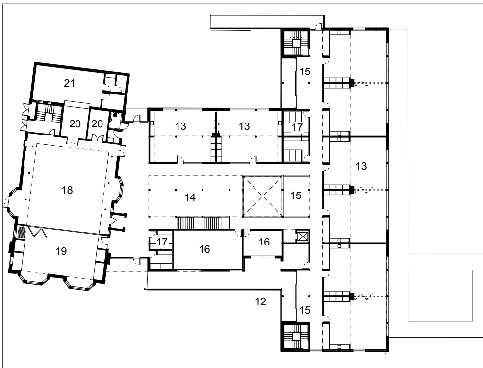
Proposed Primary Accommodation - Upper Ground Floor
